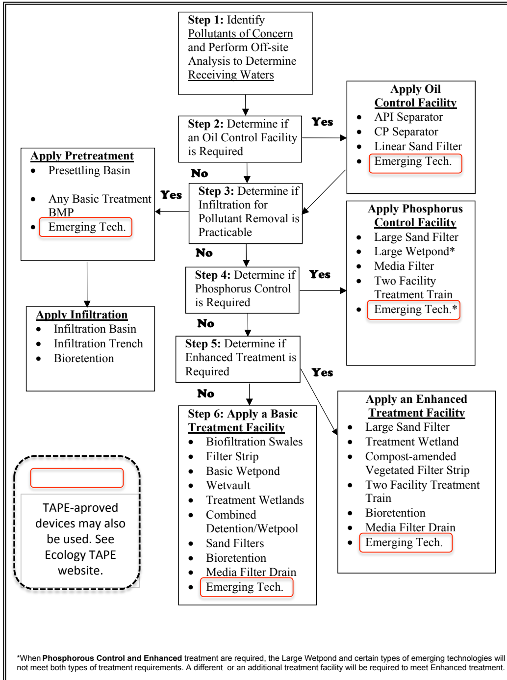
Figure 2.1.1 – Treatment Facility Selection Flow Chart
